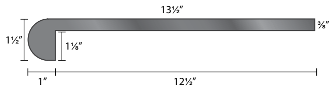
BULLNOSE PROFILE
